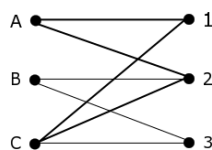
■ Figure 1 The left side of the graph (nodes A, B and C) corresponds to the elements of the set U_1 and the right side (nodes 1,2 and 3) corresponds to the elements of the set U_1 . Thus, A = \{1, 2\} , B = \{2, 3\} and C = \{1, 2, 3\} . The maximum biclique in this example has two nodes on each side. In the figure, one of the two maximum bicliques is emphasized with bold edges.
